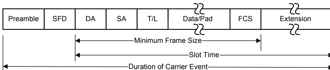
Figure 8-1. Carrier Extended Frame Format
